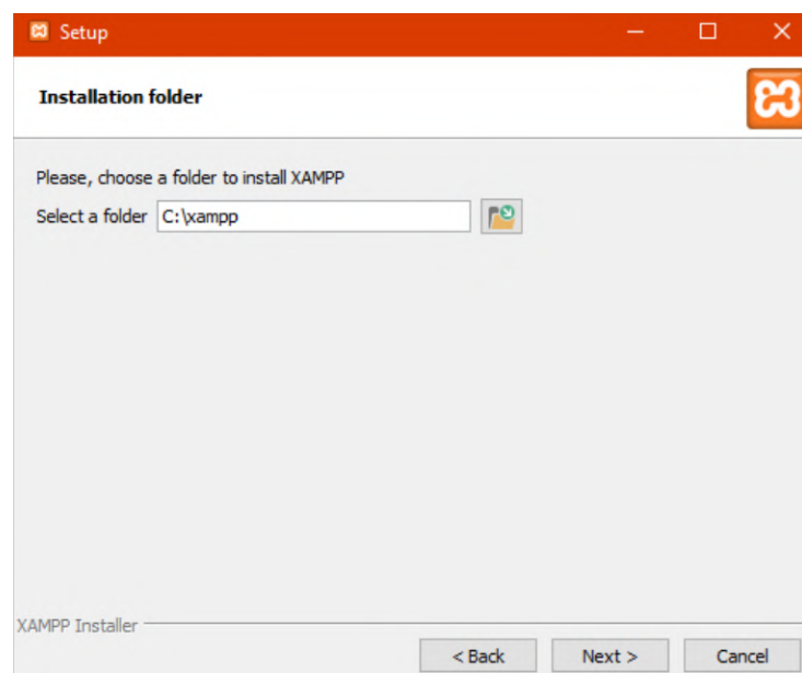
Gambar 2. 4 Instalation folder
